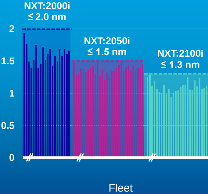
Matched Machine Overlay improvements to <1.3nm
